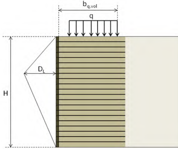
Figure 29. Illustration. Lateral deformation of a GRS structure.
