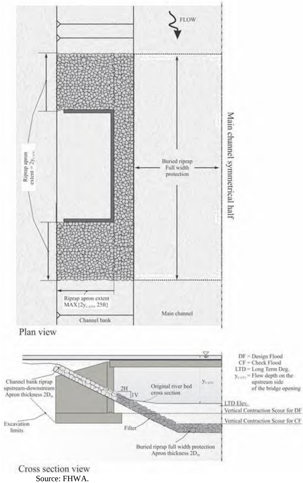
Figure 128. Illustration. Pressure flow scour countermeasure.
