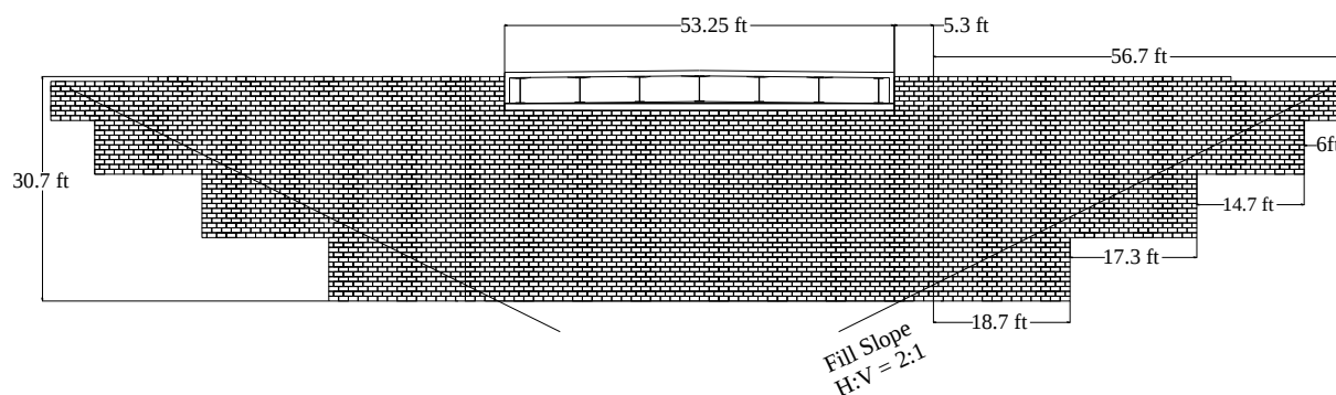
Figure 110. Illustration. Abutment and wing wall.
