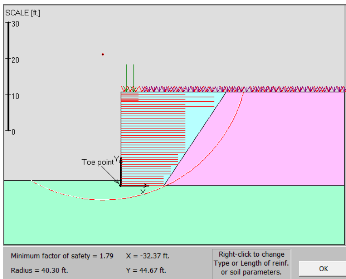
Figure 112. Screenshot. ReSSA results for global stability.
