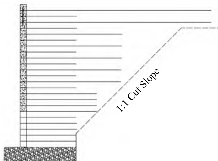
Section—Wing Wall
