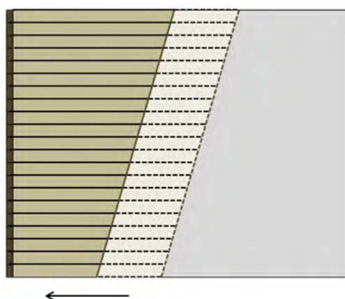
Figure 25. Illustration. External stability—direct sliding.
