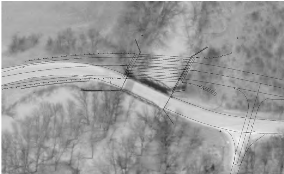
Figure 116. Photo. Aerial view of the existing site with the new Bowman Road Bridge plans superimposed.
